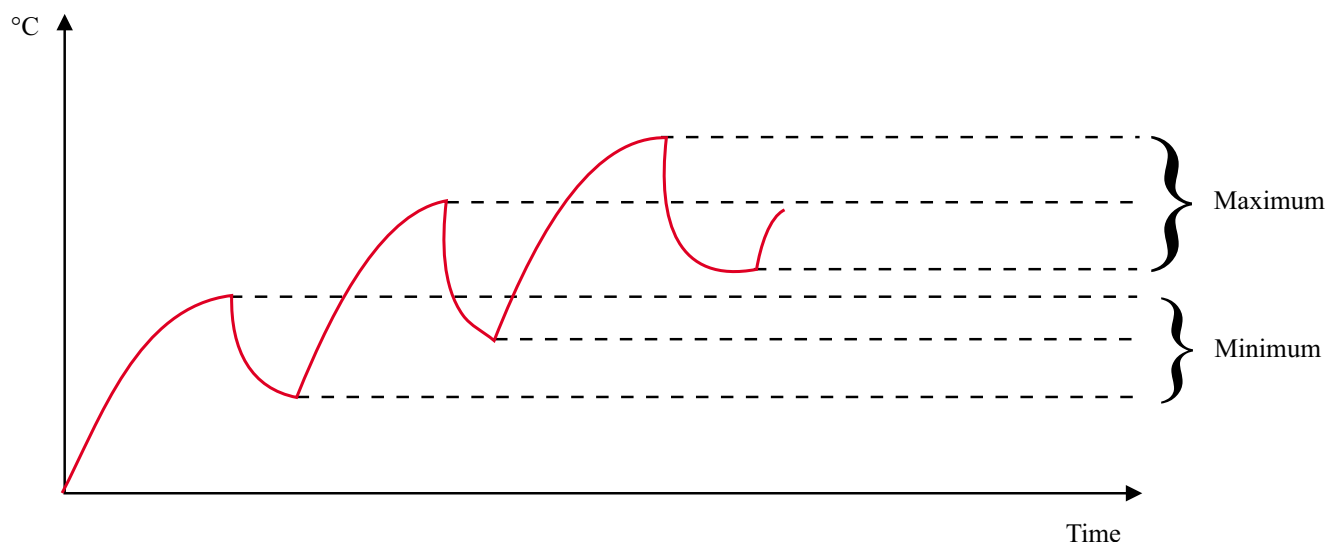
Figure J.1 - Determination of arithmetic average temperature
