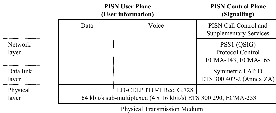
Figure 2 - Protocol stack
