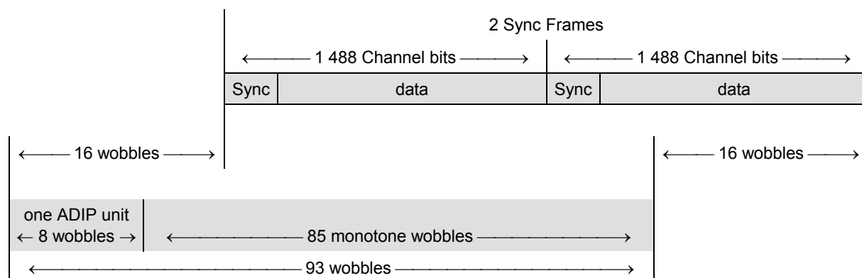
Figure 19 - General ADIP structure
