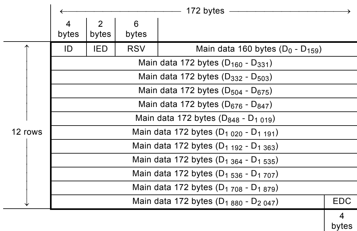
Figure 11 - Data Frame
