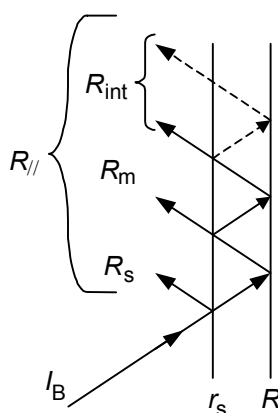
Figure C.1 – Reflectivity calibration
