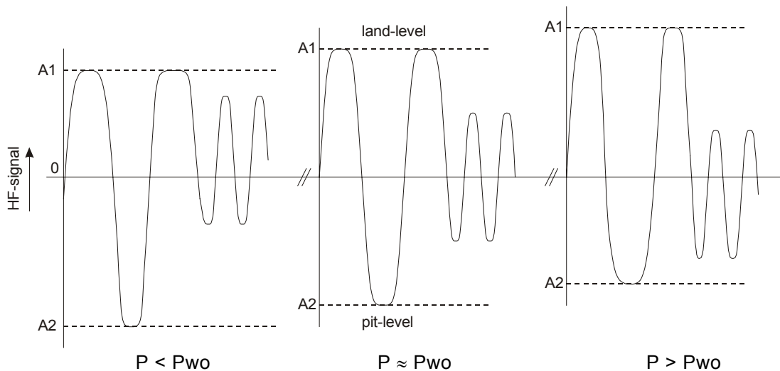
Figure I.2 - AC-coupled HF signals recorded with different writing powers
