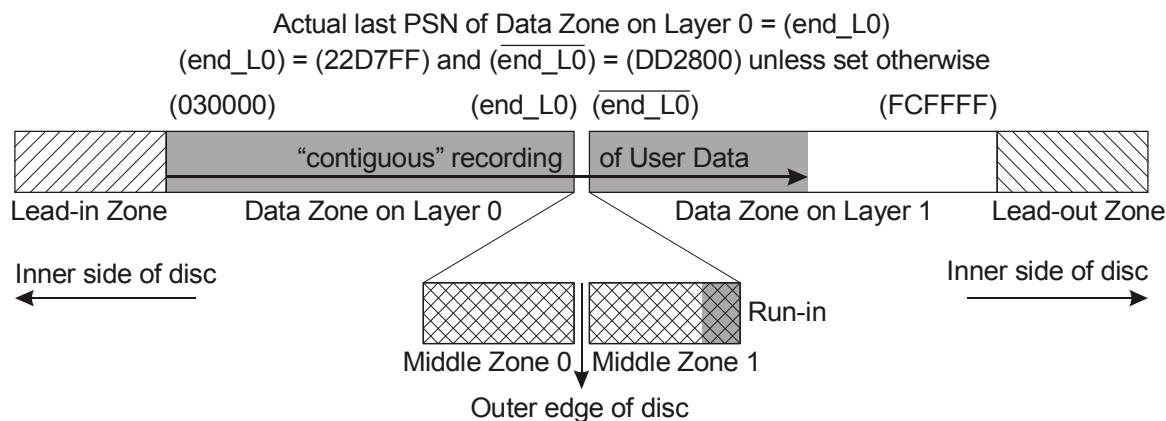
Figure 24 - Contiguity of Data Zones
