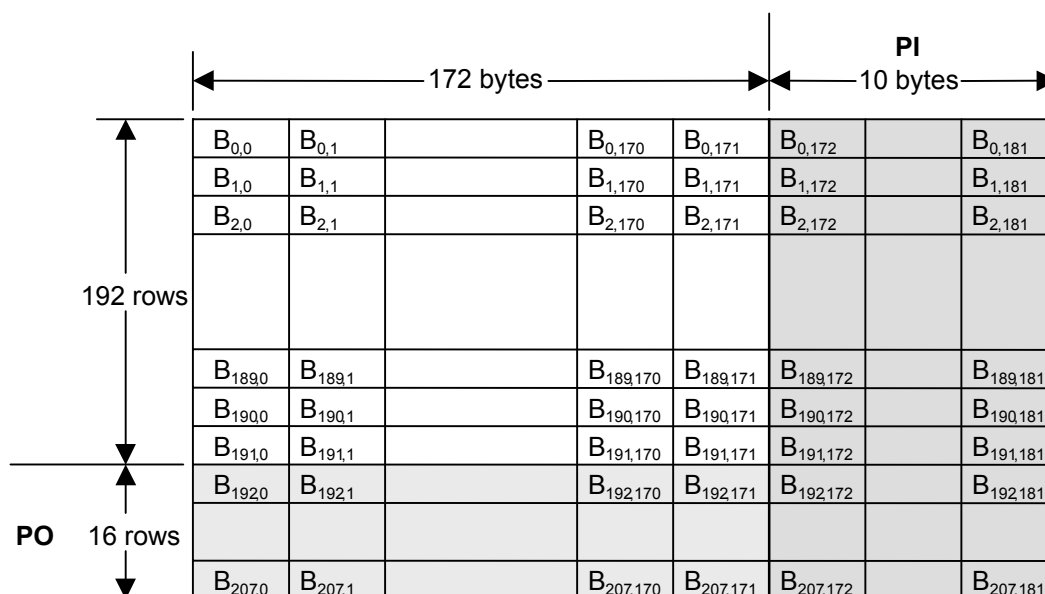
Figure 14 - ECC Block
