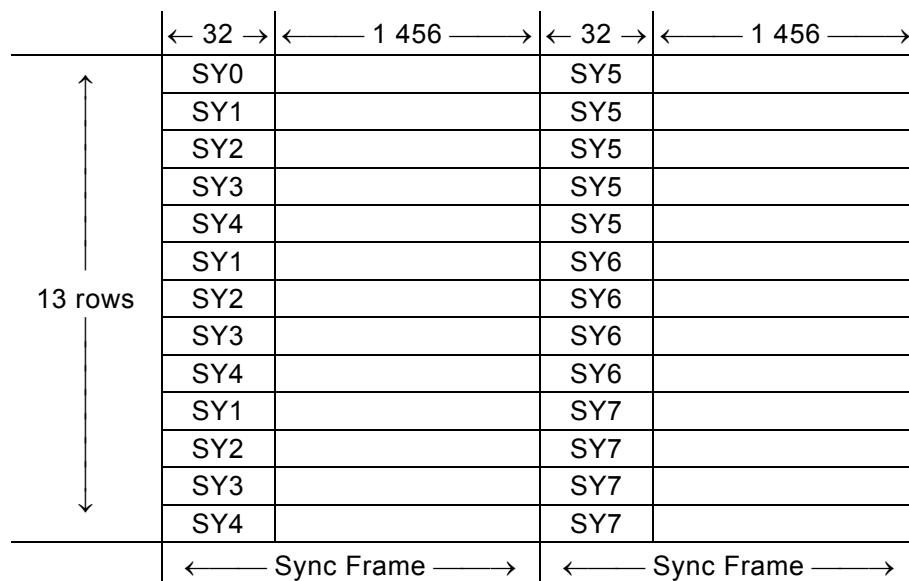
Figure 17 - Physical Sector
