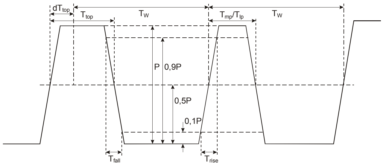
Figure G.3 – Rise Times and Fall Times
