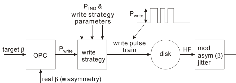
Figure I.1 - Schematic diagram of OPC procedure
