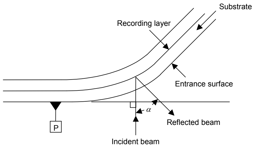
Figure 10 - Angular deviation □
