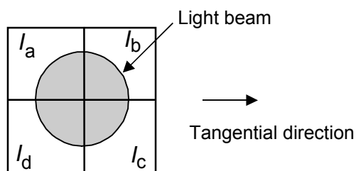
Figure 44 - Quadrant photo detector
