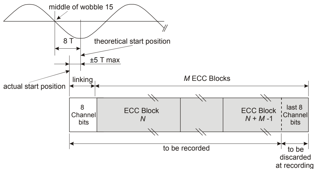
Figure 18 - Recording Unit
