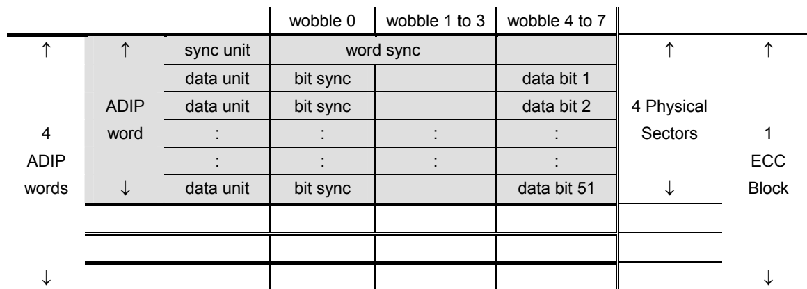
Figure 20 - ADIP word structure
