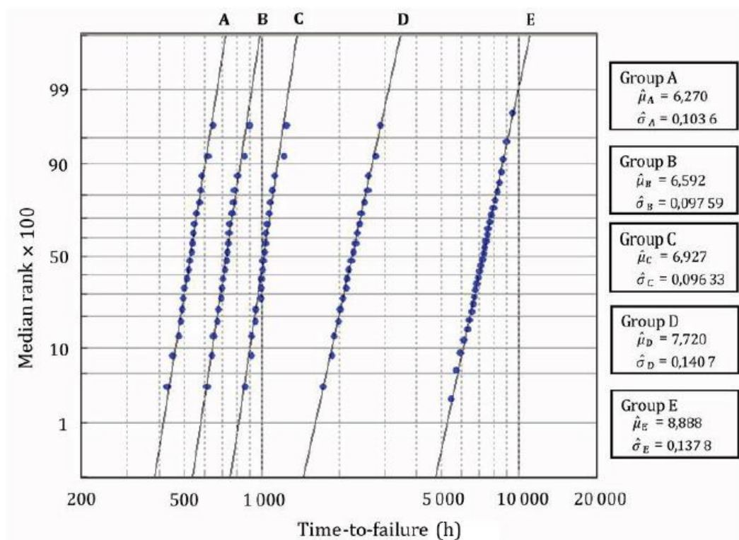
Figure B.1 — Best-fit lines of specimen groups A, B, C, D and E on lognormal paper
